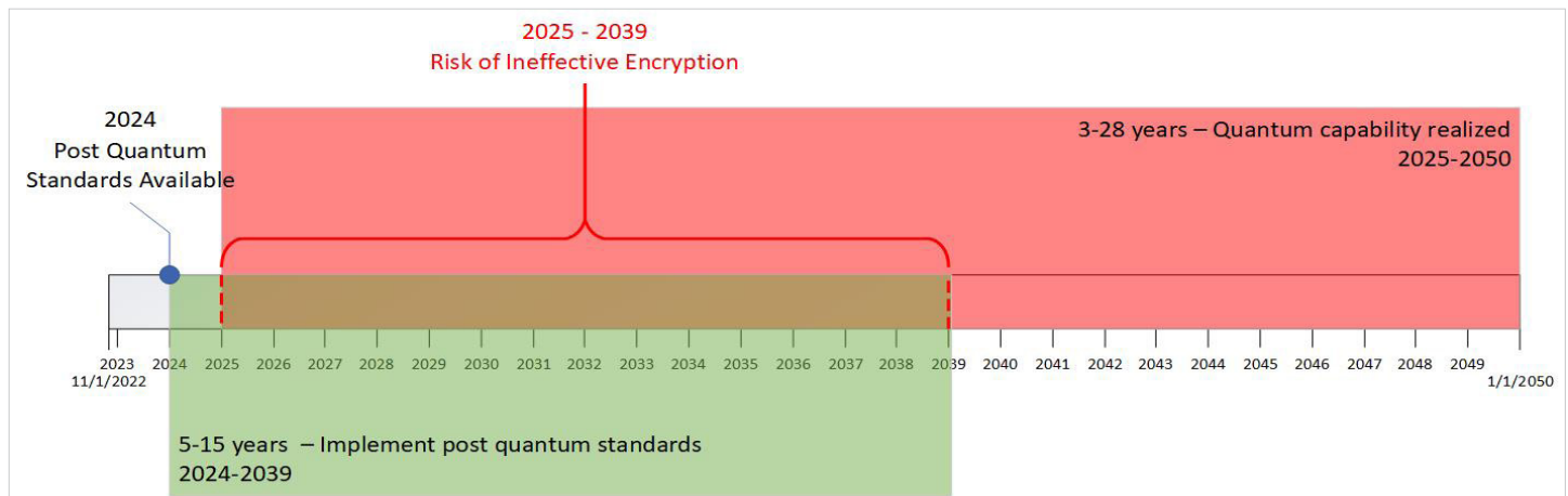
Figure 1: Quantum timeline
